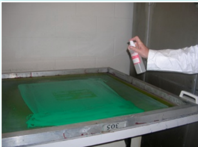
Step 1. Spray CAL-SOLV on the squeegee side of screen.
