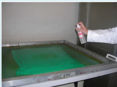
Step 1. Spray Perfect 71 on the squeegee side of screen.
